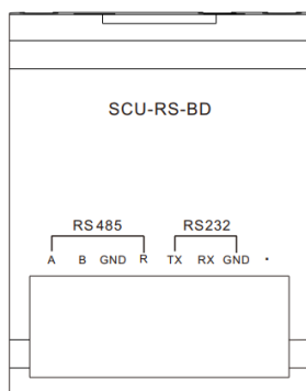
图 13-2 SCU-RS-BD模块端子丝印
