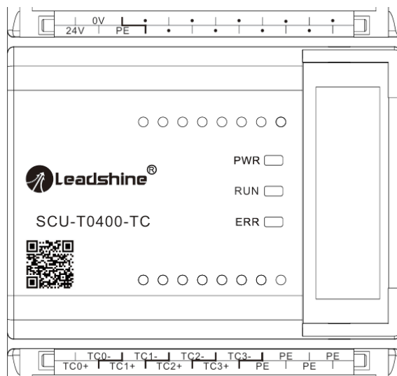
图 9-2 SCU- T0400-TC模块端子丝印
